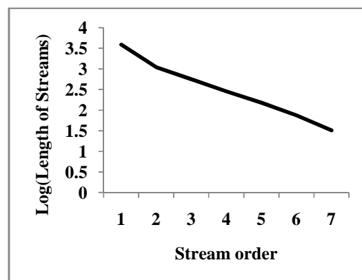
Fig 4: Relationship between Logarithm of Length of Stream versus Stream order
