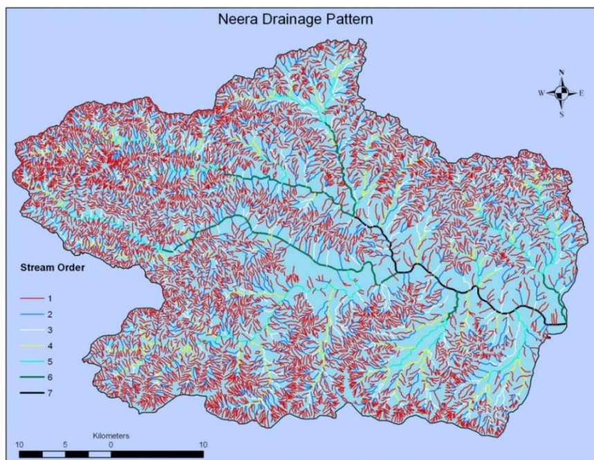
Fig 2. Drainage pattern of upper Neera river
